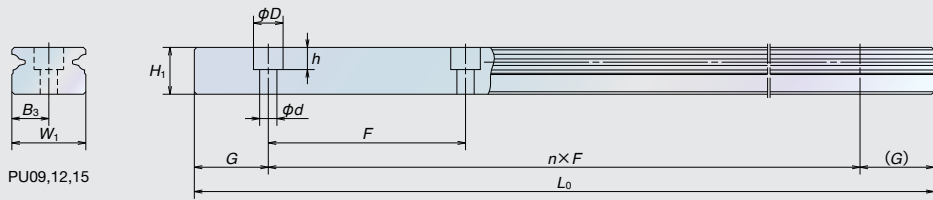
Fig. 11 Rail of interchangeable types (PU Series)
